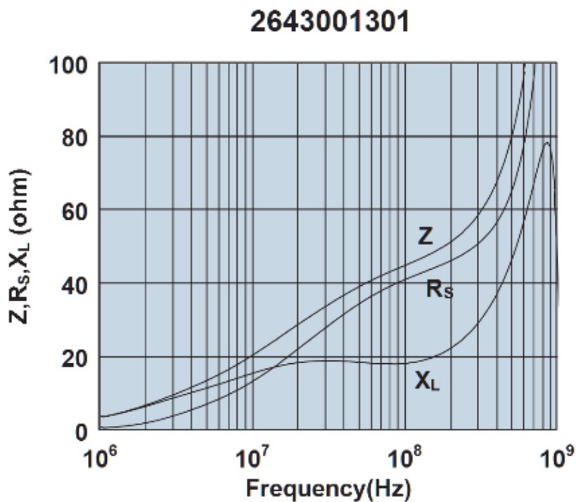
Impedance, reactance, and resistance vs. frequency.
